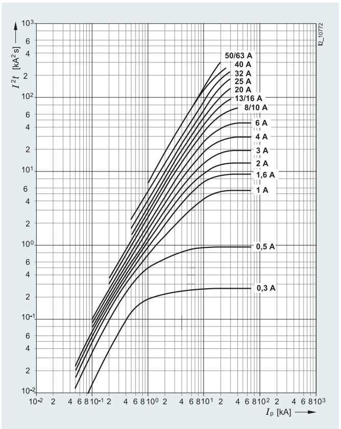
Characteristic D
