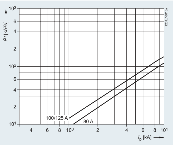
Characteristic B
