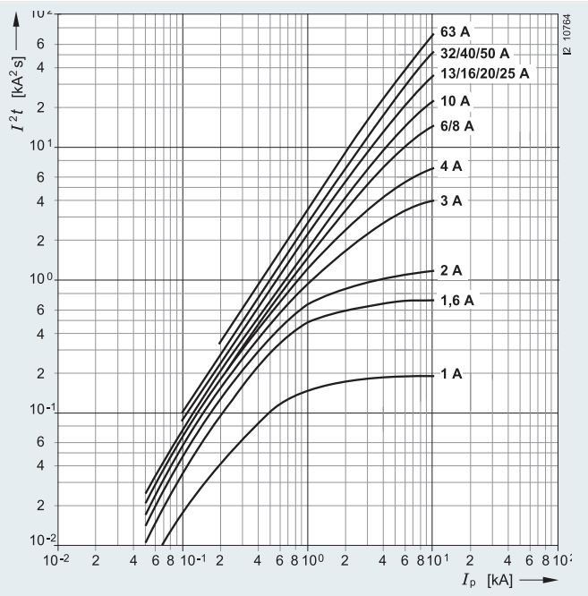
Characteristic A
