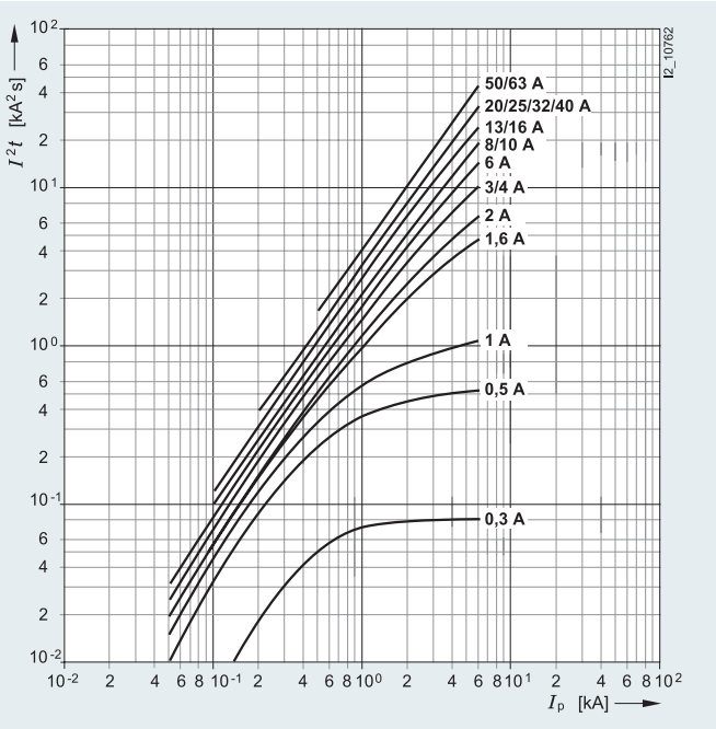
Characteristic C
