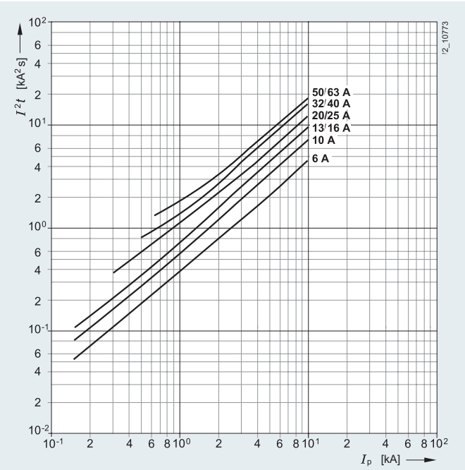
Characteristic B
