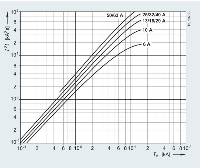
Characteristic B
