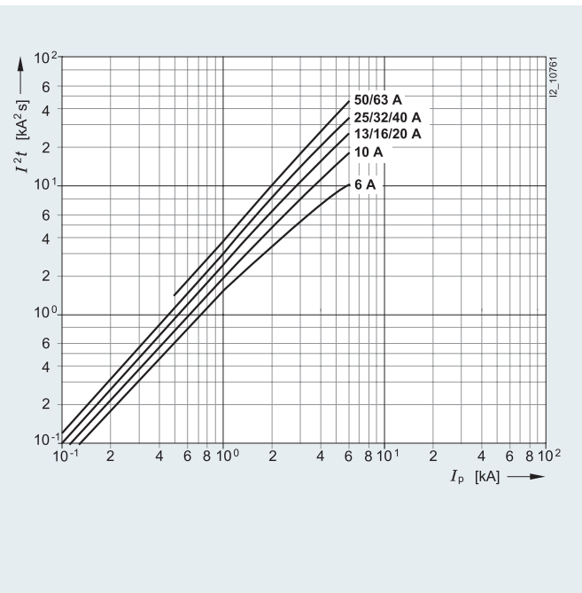
Characteristic B
