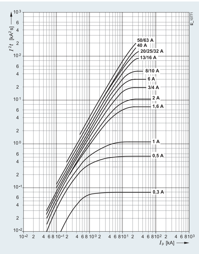
Characteristic C
