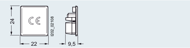
5ST3 750-0HG
