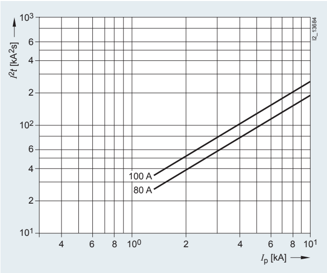
Characteristic D
