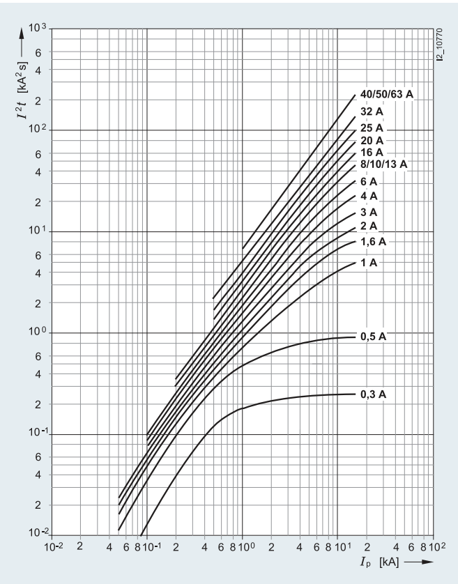
Characteristic D
