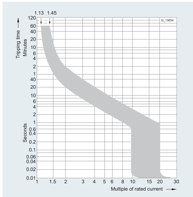
Tripping characteristic D
