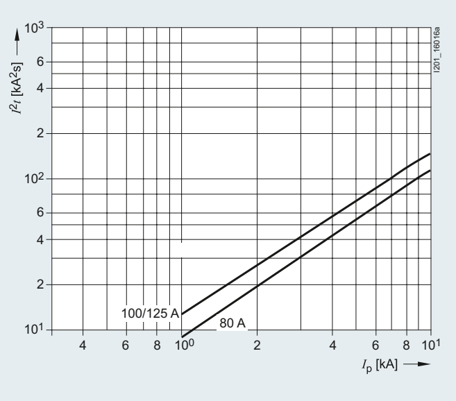
Characteristic C
