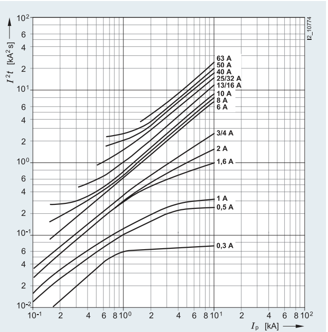
Characteristic C
