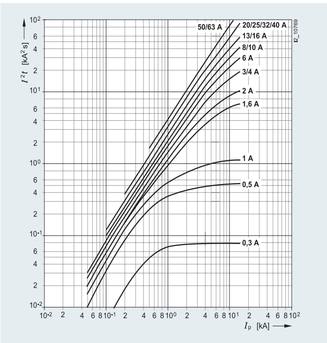
Characteristic C
