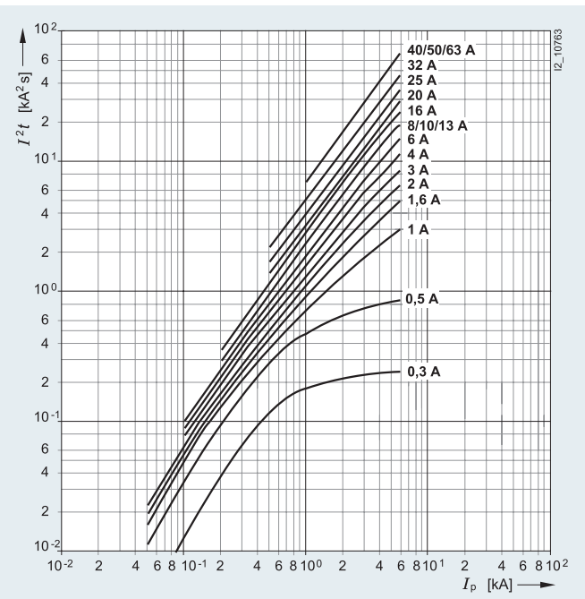
Characteristic D
