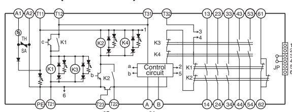
G9SA-321-T□ (24 VAC/VDC)
