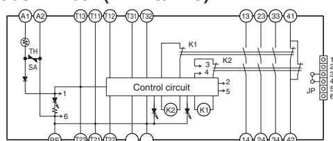
G9SA-TH301 (24 VAC/VDC)
