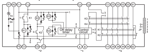
G9SA-TH301 (24 VAC/VDC)
